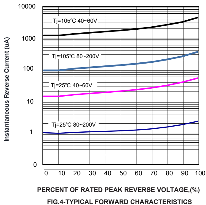
FIG.4-TYPICAL FORWARD CHARACTERISTICS
